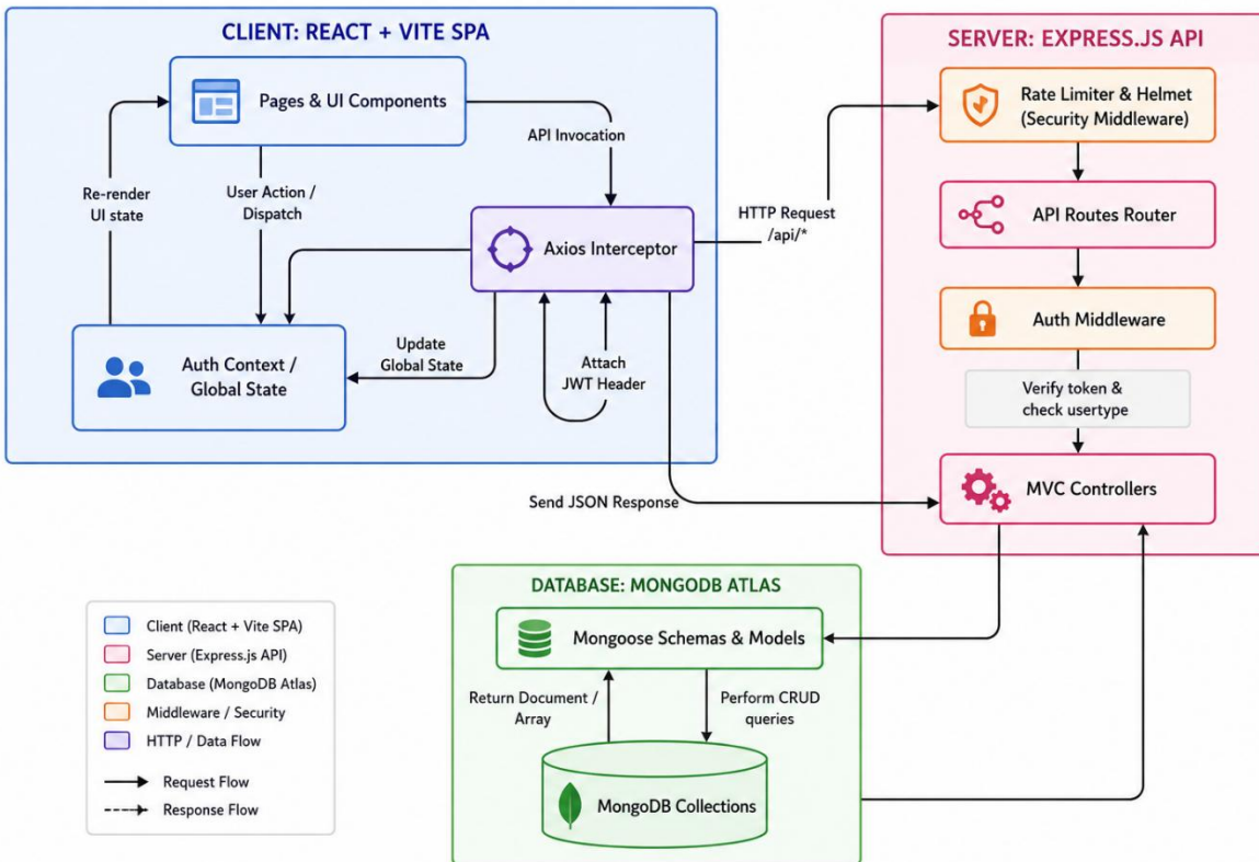
Figure 1: ShopEZ architecture and request/response data flow across the React client, Express API, and MongoDB Atlas database.
